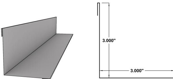
Inside Angle *Available in 1" to 4"
