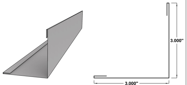
Outside Angle *Available in 1" to 4"
